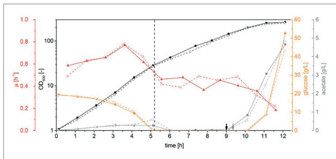
Figure 2: Overview of the cultivation in the BIOSTAT® B-DCU (solid lines) with a UniVessel® Glass 5 L compared to a former cultivation (dashed lines) with a UniVessel® Glass 5 L. Shown is the optical density at 600 nm (black), growth rate (red), acetate (grey) and glucose (orange) concentration. The start of the feed is indicated by the dashed line and the bolus feed 2 is indicated by the arrow.
