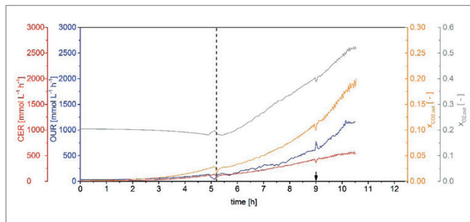
Figure 4: Exhaust gas measurement of the cultivation in the BIOSTAT® B-DCU with a UniVessel® Glass 5 L for oxygen (grey) and carbon dioxide (orange) as well as calculated oxygen uptake rate (blue) and carbon dioxide evolution rate (red). The start of the feed is indicated by the dashed line and the bolus feed 2 is indicated by the arrow. Exhaust gas measurement was stopped when the measuring range of \text{O}_2 (50%) and \text{CO}_2 (20%) was exceeded after 10.5h.
