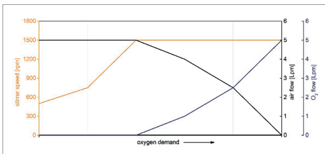
Figure 1: Schematic p\text{O}_2 cascade of both cultivations. Starting with a constant air gas flow of 5 lpm, p\text{O}_2 was controlled by increasing tip speed to 1500 rpm and supplementing oxygen.
