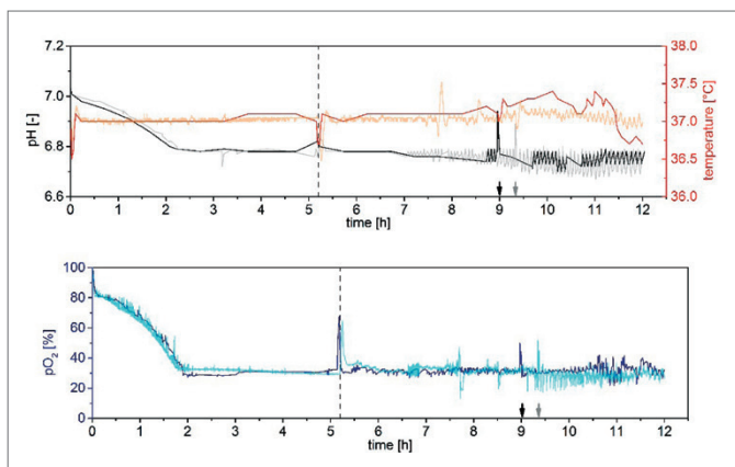
Figure 3: Process control of both cultivations. The p\text{O}_2 was controlled by changing the tip speed and supplementing oxygen (fig. 1). Additionally, pH and temperature were also controlled. BIOSTAT® B-DCU data were colored and data from a former cultivation were light-colored, respectively.
